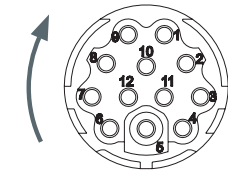
mating view
