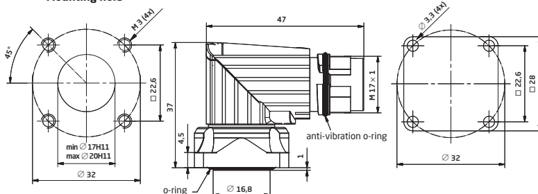
Mounting hole
