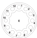
mating view
